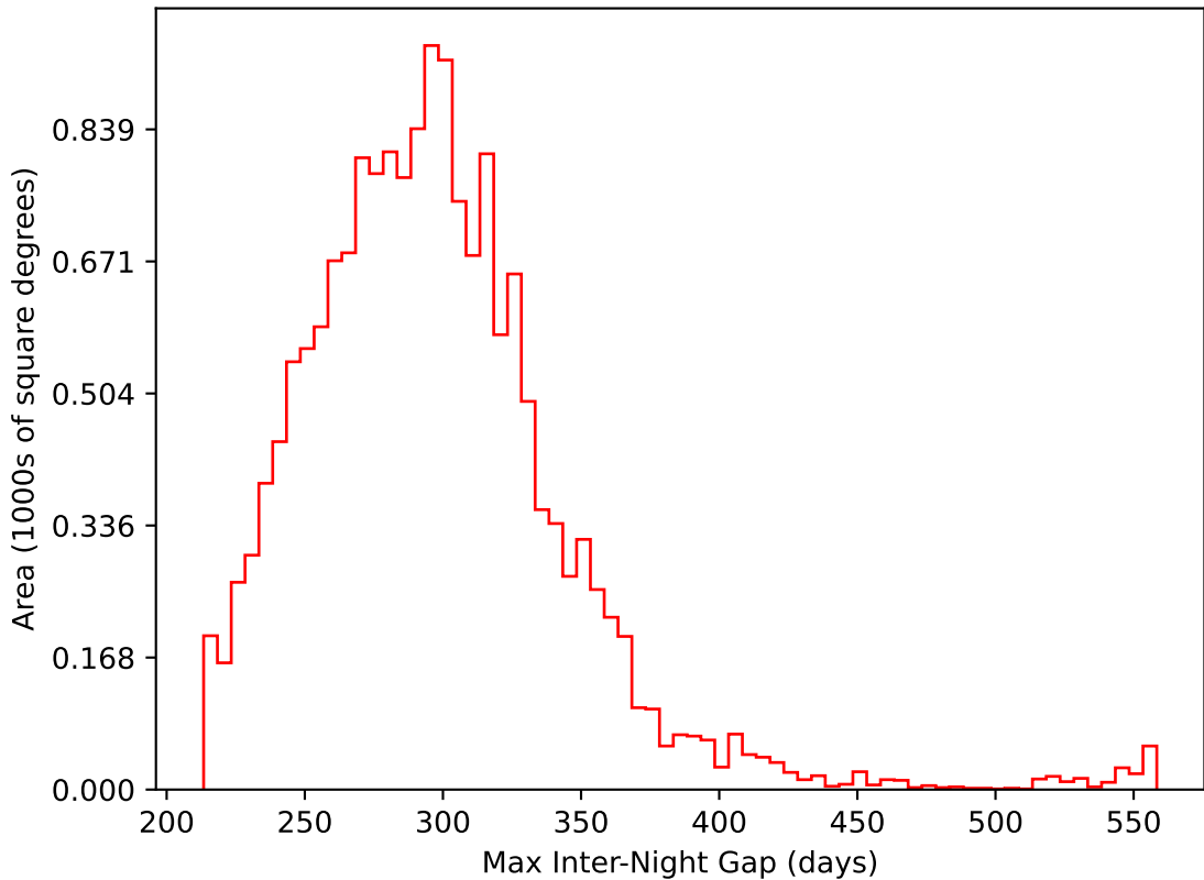
too_elab_heavy_r128_d2_griz_v3.4_10yrs WFD i band: Max Inter-Night Gap
