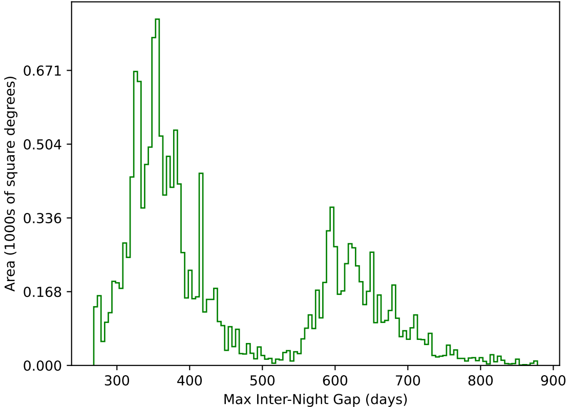
too_elab_heavy_r128_d2_griz_v3.4_10yrs WFD g band: Max Inter-Night Gap
