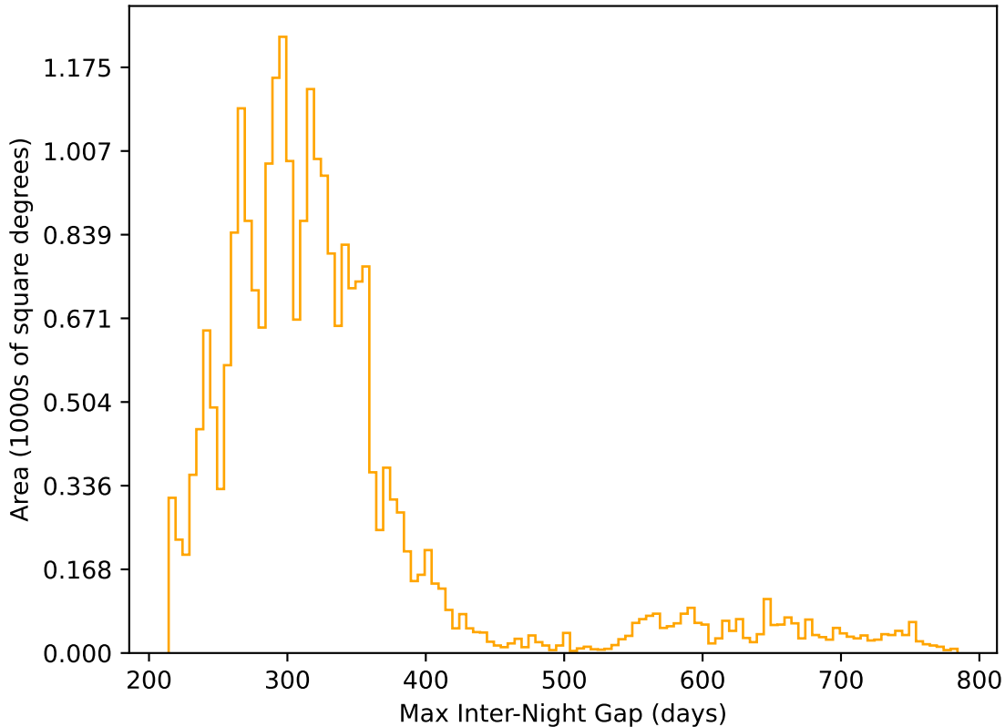
too_elab_heavy_r128_d2_griz_v3.4_10yrs All sky r band: Max Inter-Night Gap
