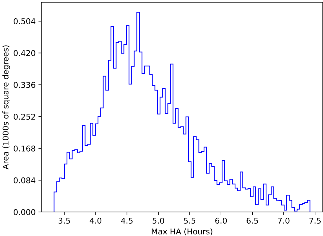
too_elab_heavy_r128_d2_griz_v3.4_10yrs WFD y band: Max HA
