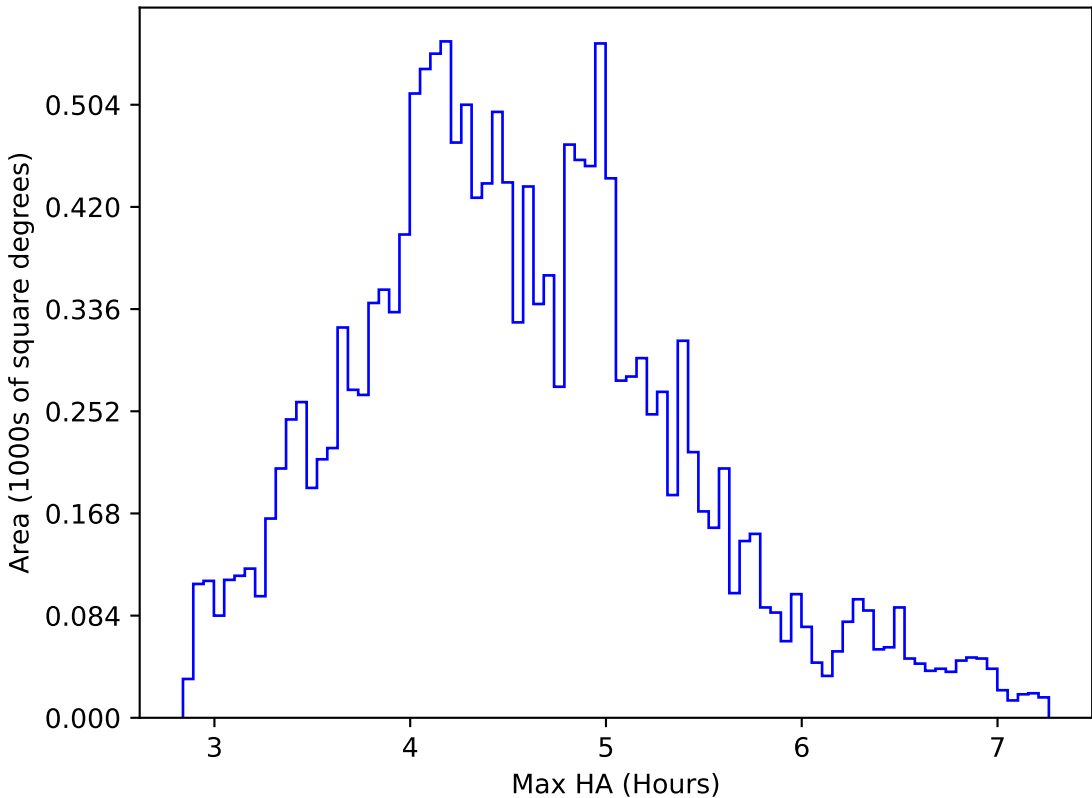
too_elab_heavy_r128_d2_griz_v3.4_10yrs WFD r band: Max HA
