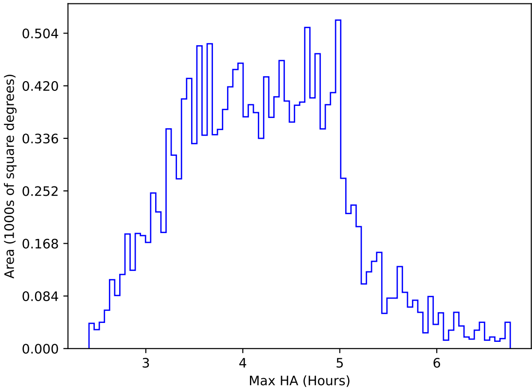
too_elab_heavy_r128_d2_griz_v3.4_10yrs WFD g band: Max HA
