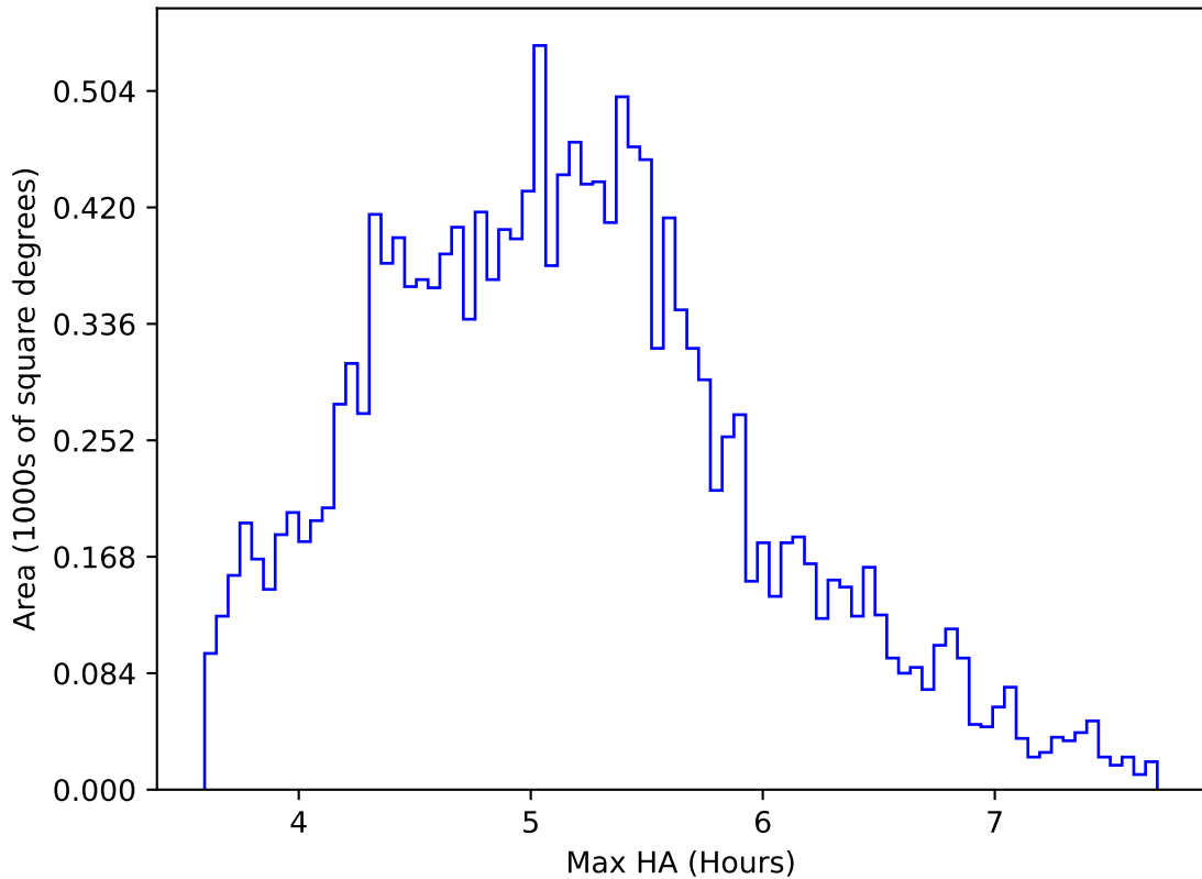
too_elab_heavy_r128_d2_griz_v3.4_10yrs WFD all bands: Max HA
