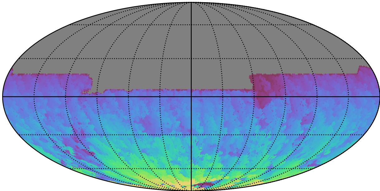
too_elab_heavy_r128_d2_griz_v3.4_10yrs All sky y band: Max HA
