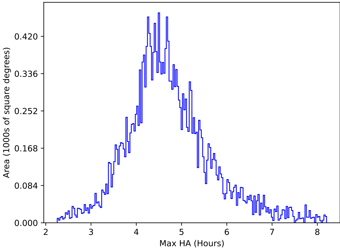
too_elab_heavy_r128_d2_griz_v3.4_10yrs All sky y band: Max HA
