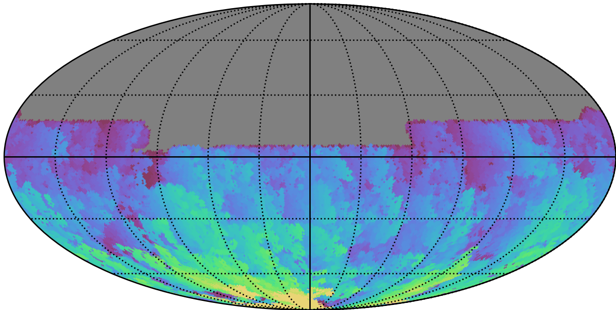
too_elab_heavy_r128_d2_griz_v3.4_10yrs All sky u band: Max HA
