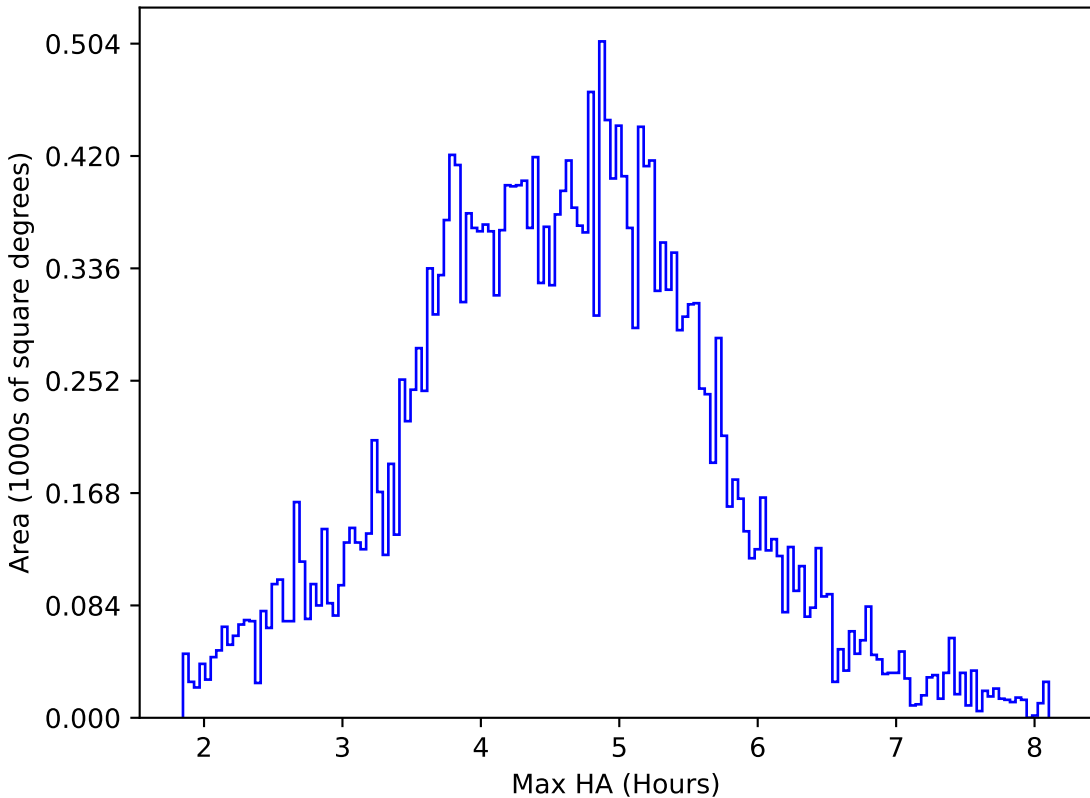
too_elab_heavy_r128_d2_griz_v3.4_10yrs All sky i band: Max HA
