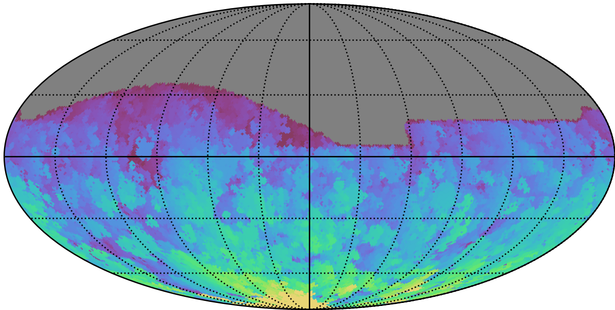
too_elab_heavy_r128_d2_griz_v3.4_10yrs All sky g band: Max HA
