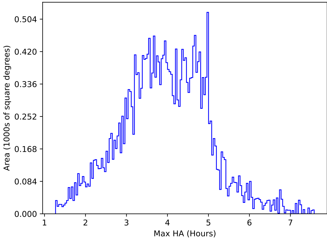
too_elab_heavy_r128_d2_griz_v3.4_10yrs All sky g band: Max HA
