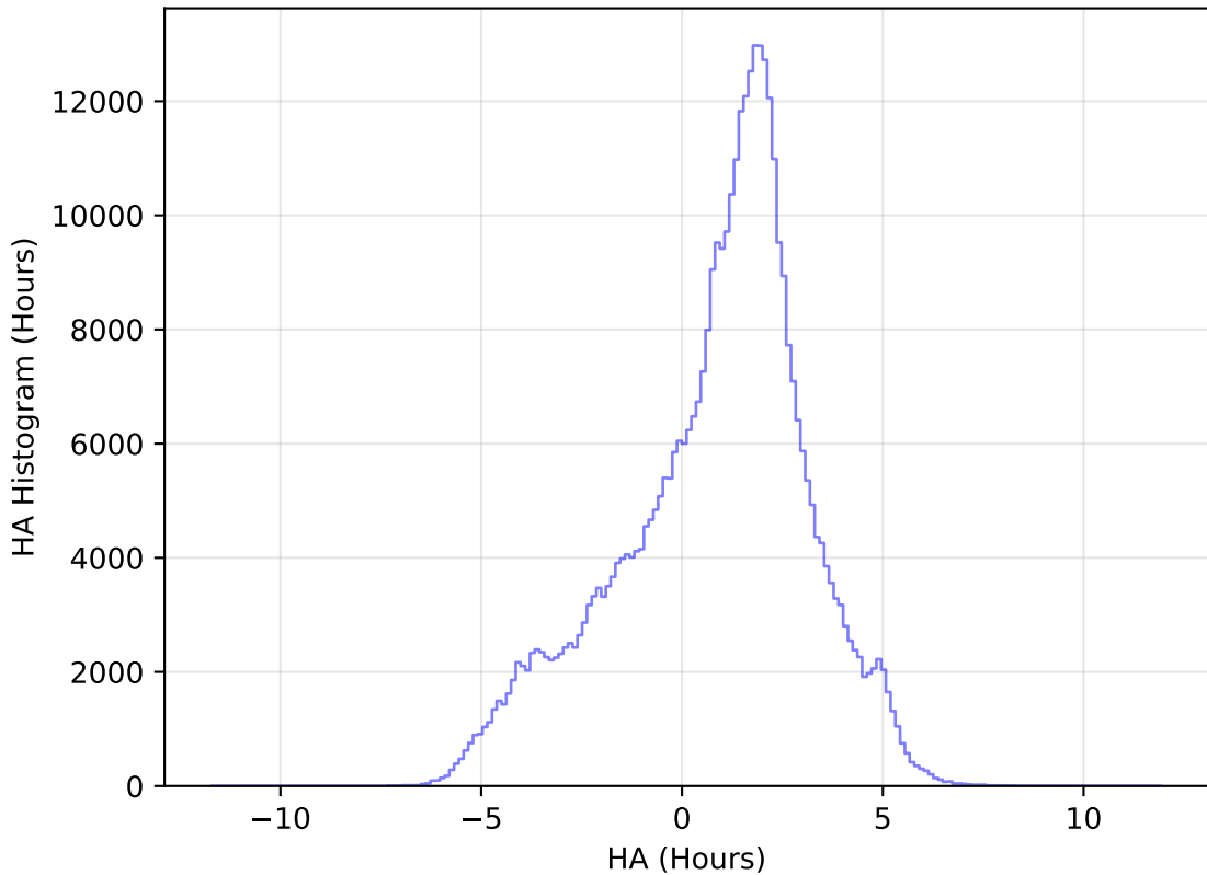
too_elab_heavy_r128_d2_griz_v3.4_10yrs WFD z band: HA Histogram
