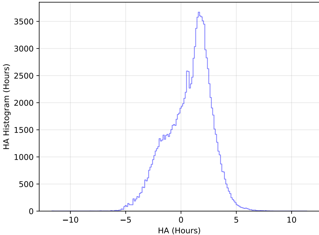
too_elab_heavy_r128_d2_griz_v3.4_10yrs WFD u band: HA Histogram
