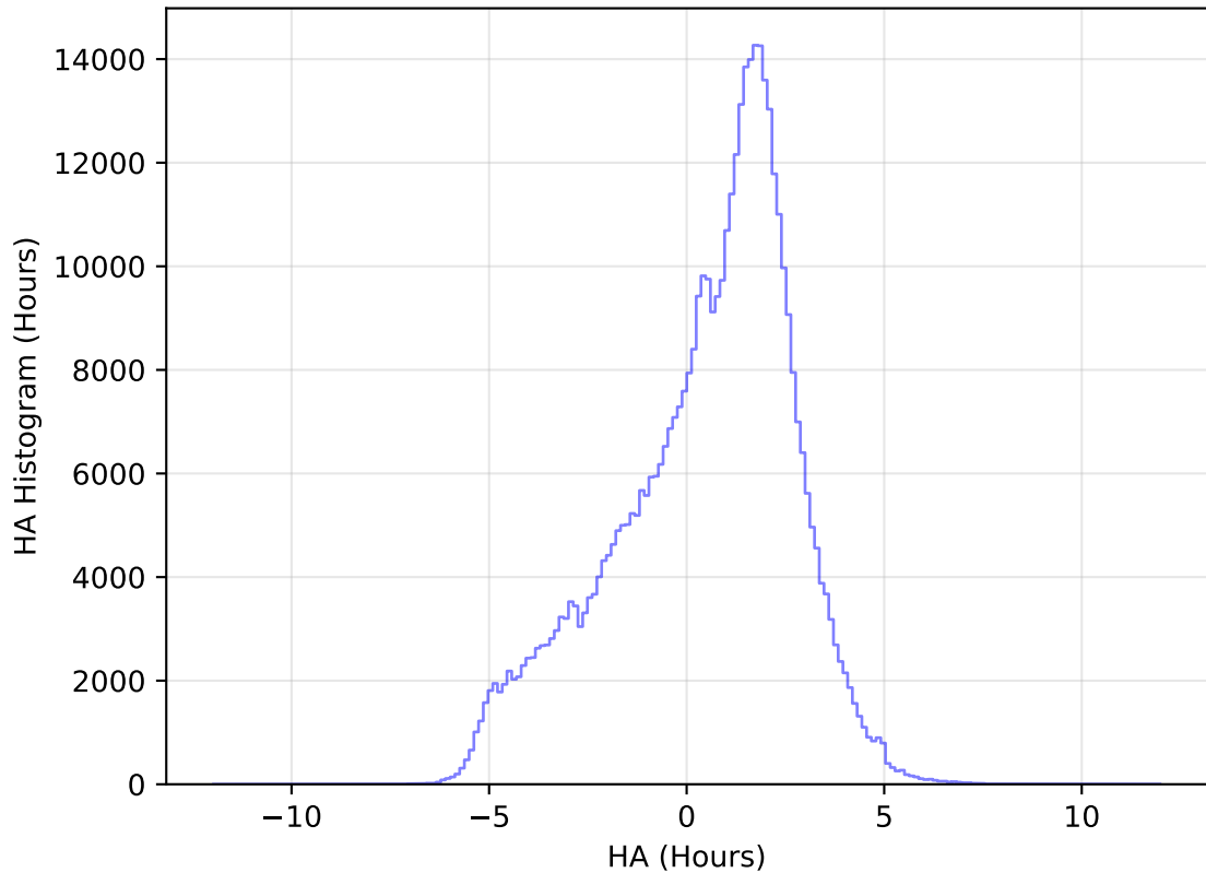
too_elab_heavy_r128_d2_griz_v3.4_10yrs WFD r band: HA Histogram
