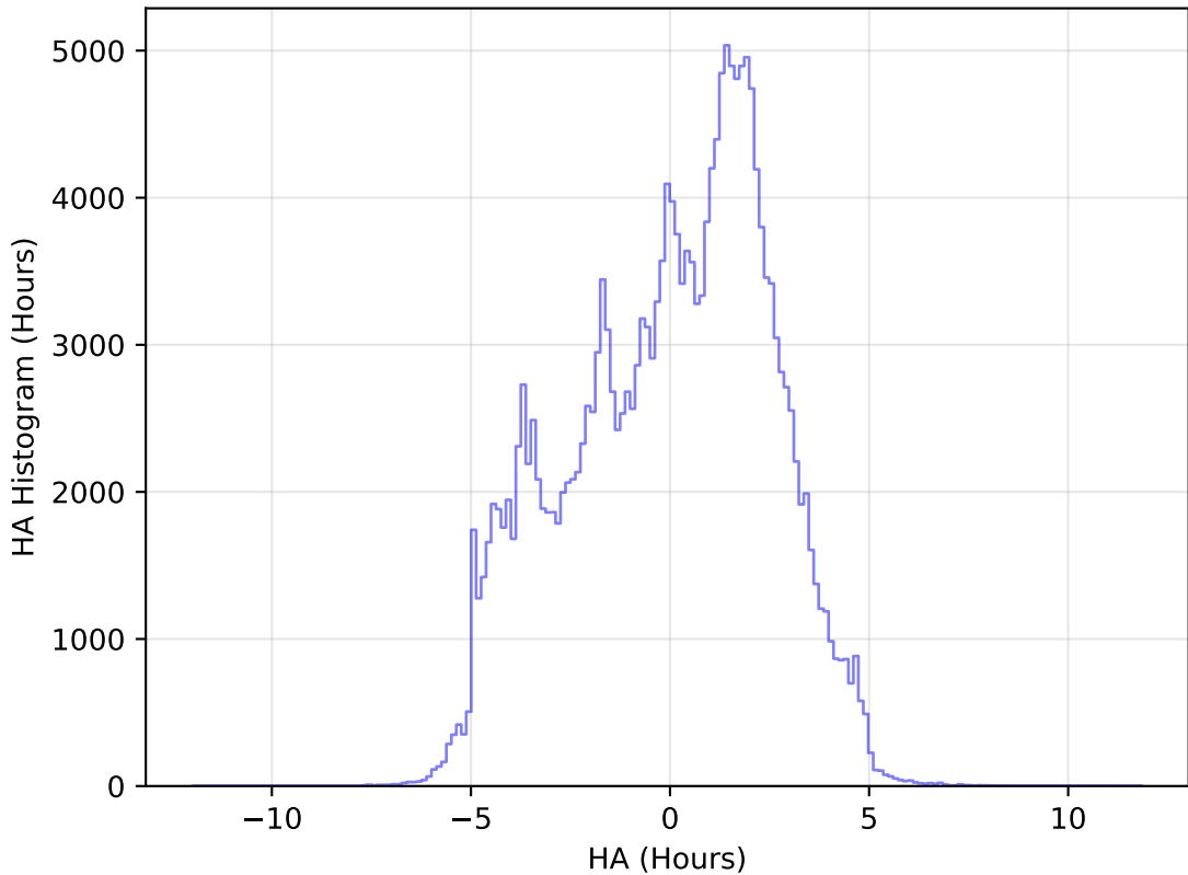
too_elab_heavy_r128_d2_griz_v3.4_10yrs WFD g band: HA Histogram
