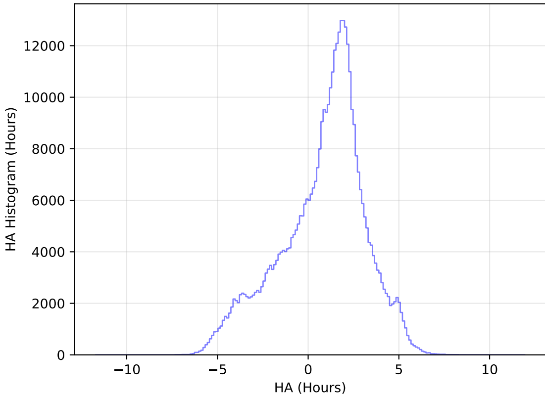
too_elab_heavy_r128_d2_griz_v3.4_10yrs All sky z band: HA Histogram
