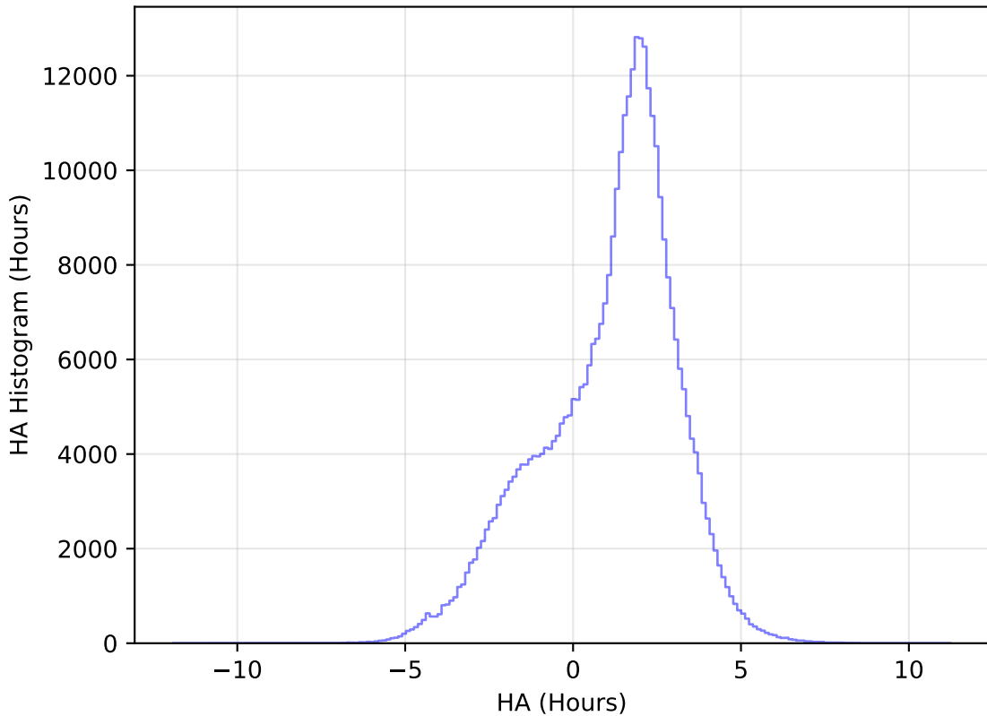
too_elab_heavy_r128_d2_griz_v3.4_10yrs All sky y band: HA Histogram
