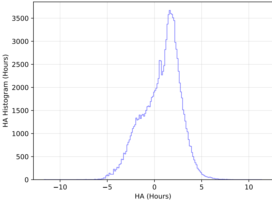
too_elab_heavy_r128_d2_griz_v3.4_10yrs All sky u band: HA Histogram
