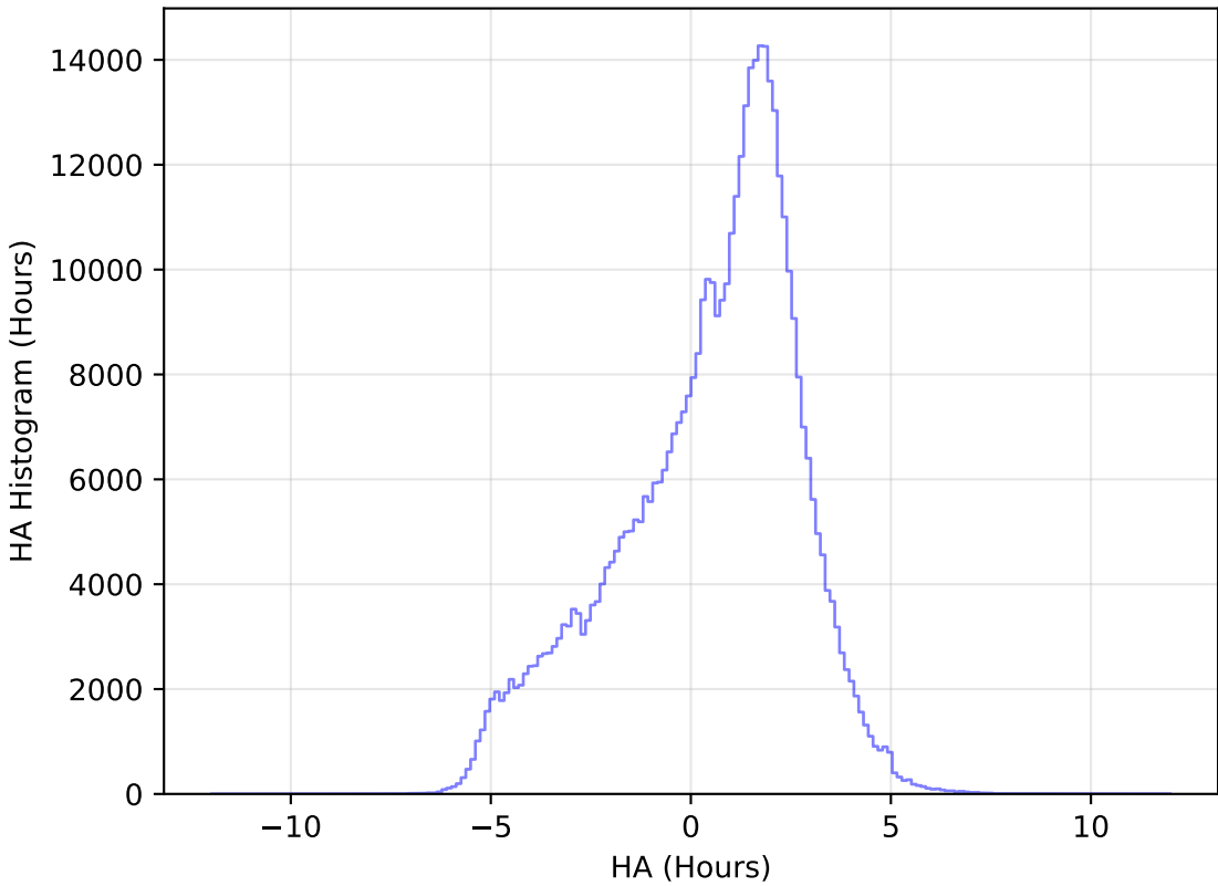
too_elab_heavy_r128_d2_griz_v3.4_10yrs All sky r band: HA Histogram
