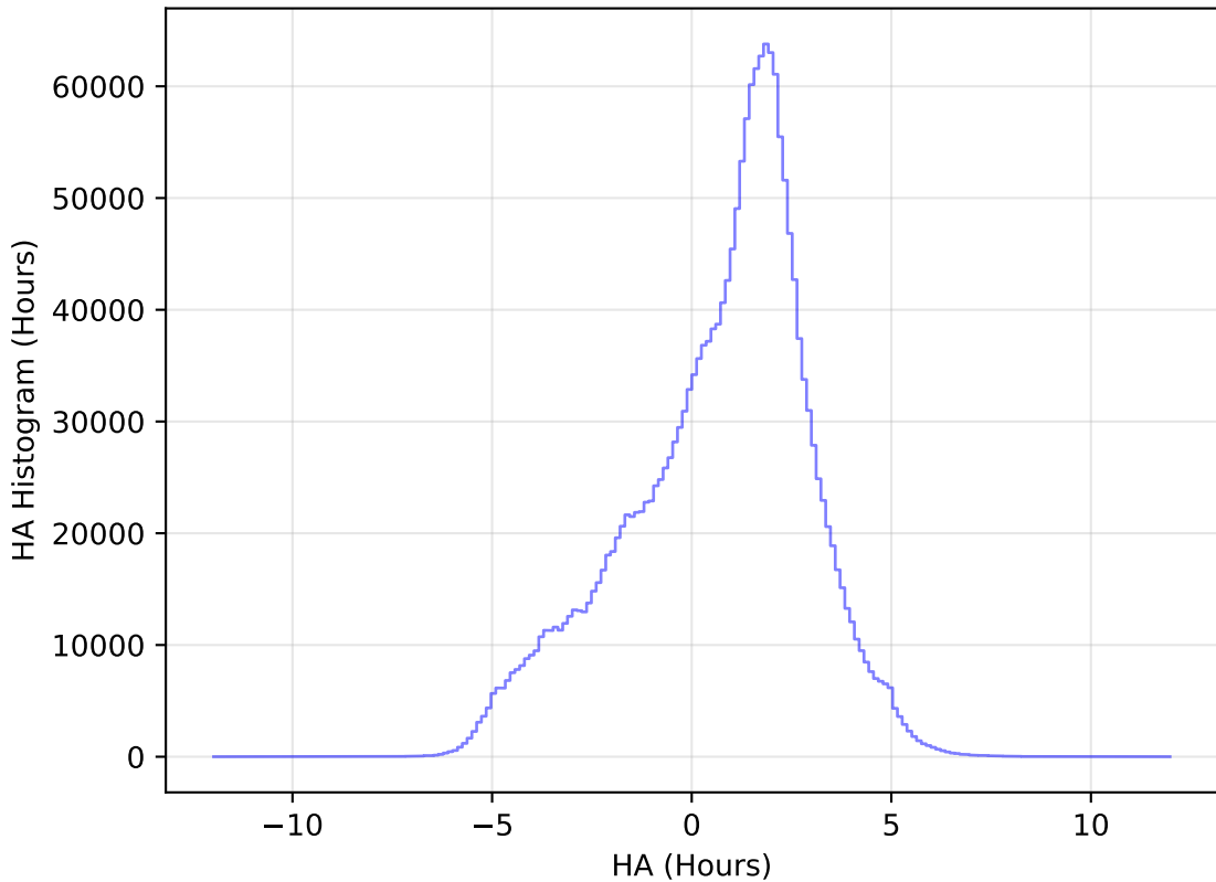
too_elab_heavy_r128_d2_griz_v3.4_10yrs All sky all bands: HA Histogram
