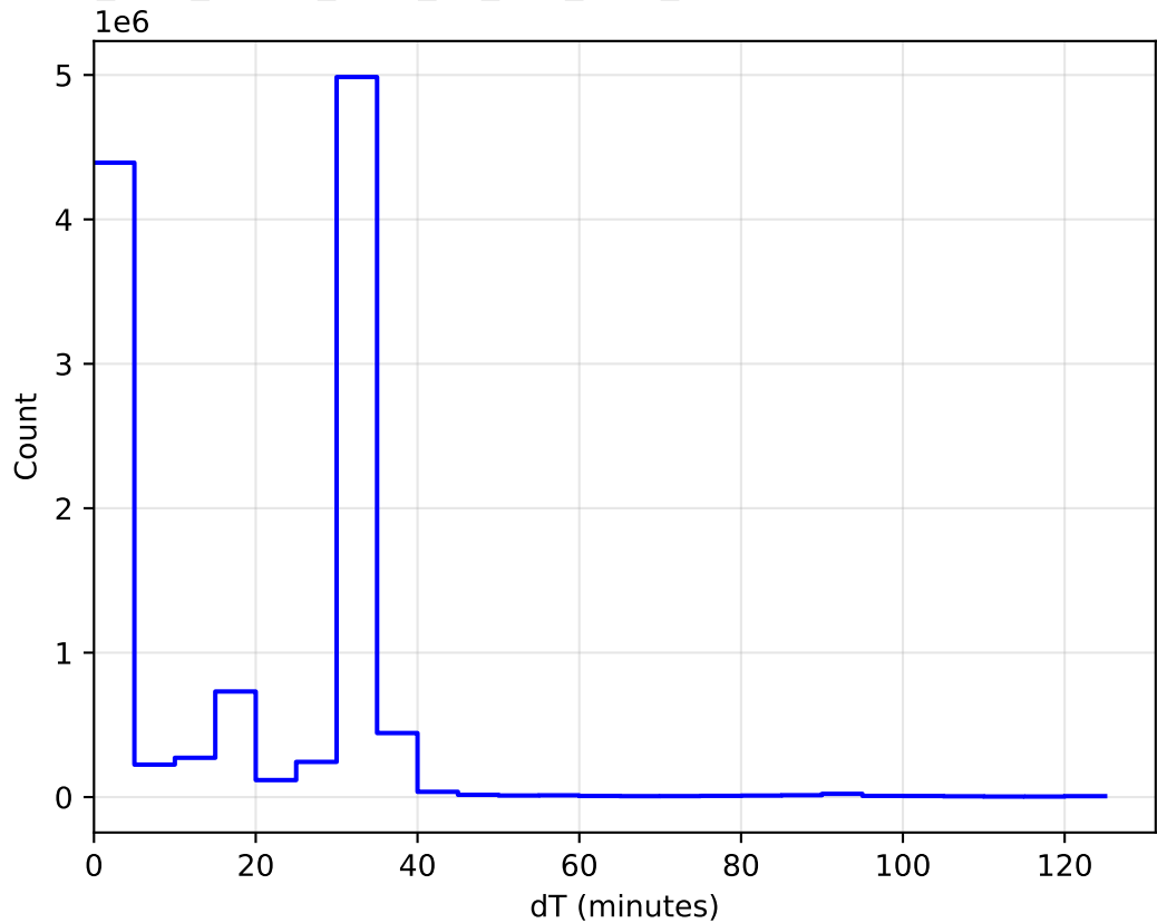
too_elab_heavy_r128_d2_griz_v3.4_10yrs WFD: DeltaT Histogram
