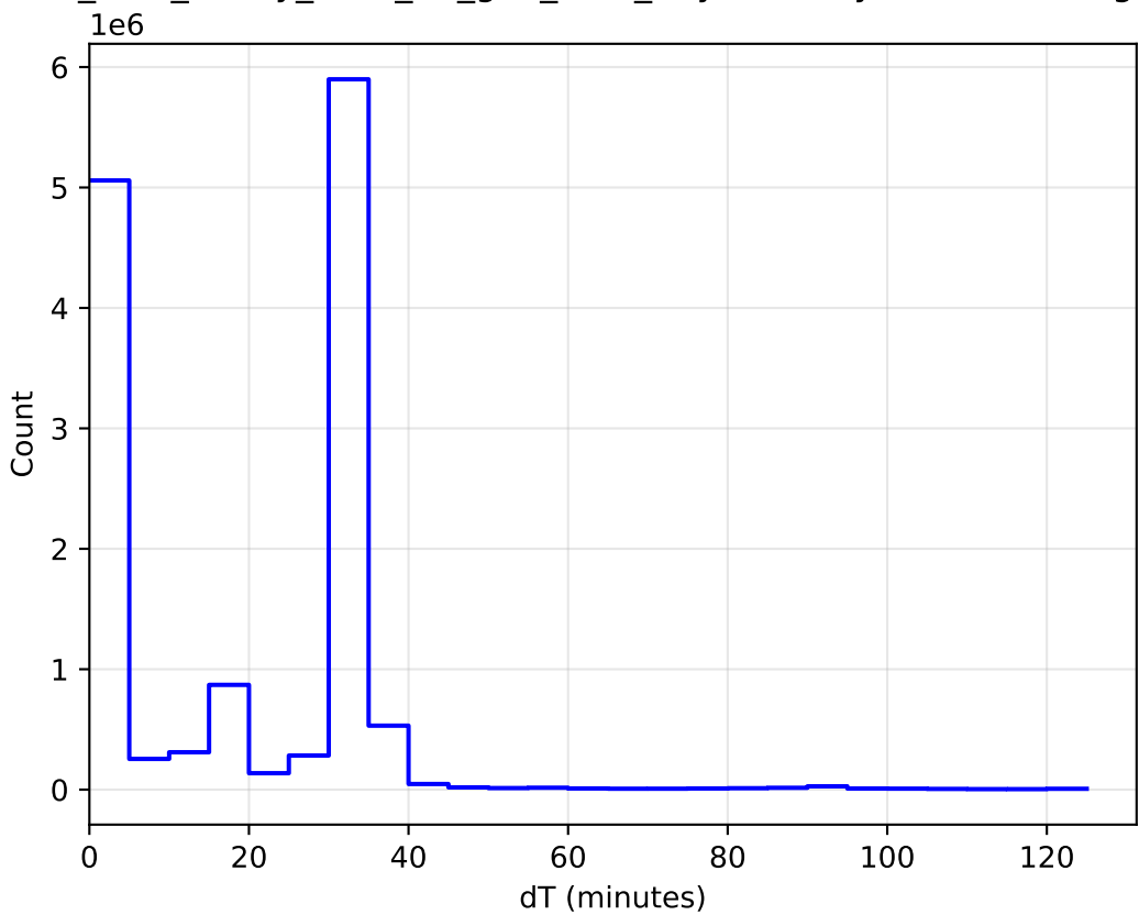
too_elab_heavy_r128_d2_griz_v3.4_10yrs All sky: DeltaT Histogram
