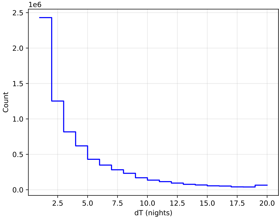
too_elab_heavy_r128_d2_griz_v3.4_10yrs WFD all bands: DeltaNight Histogram
