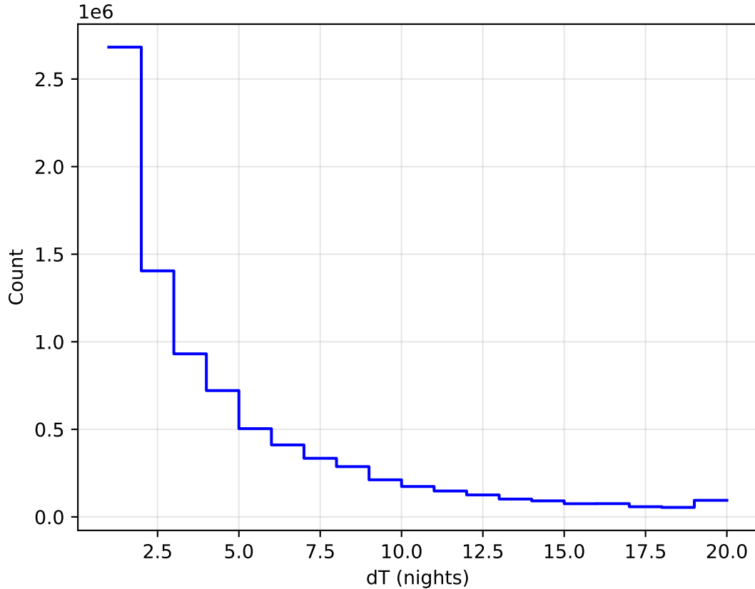
too_elab_heavy_r128_d2_griz_v3.4_10yrs All sky all bands: DeltaNight Histogram
