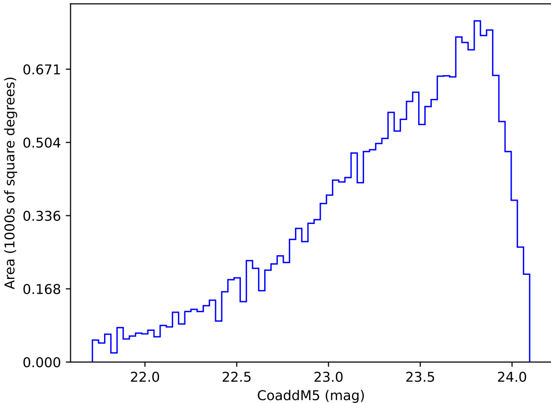
too_elab_heavy_r128_d2_griz_v3.4_10yrs Yr 3-4 y band: CoaddM5
