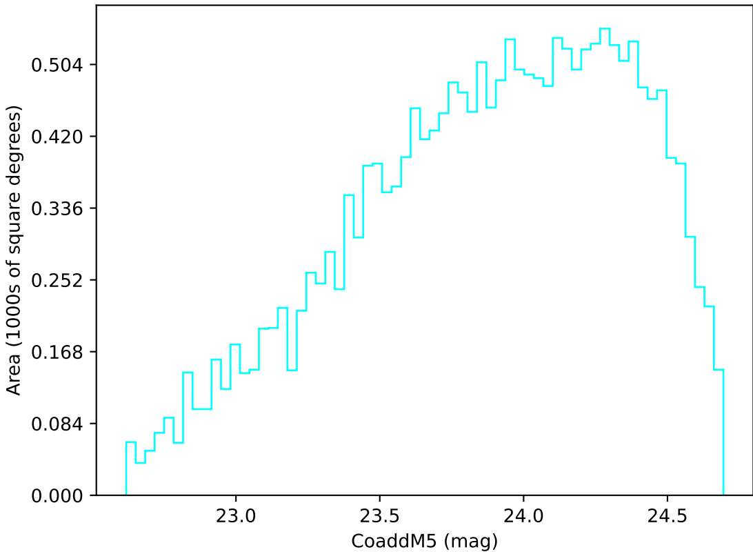
too_elab_heavy_r128_d2_griz_v3.4_10yrs Yr 3-4 u band: CoaddM5
