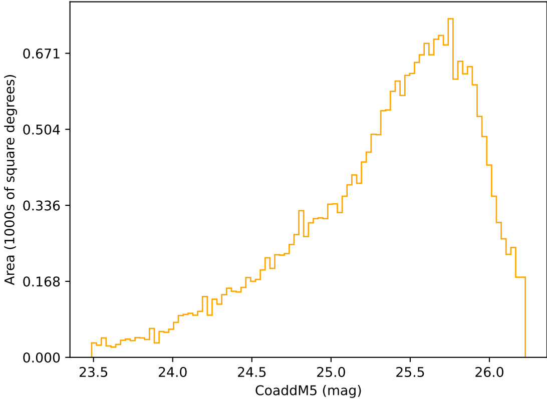
too_elab_heavy_r128_d2_griz_v3.4_10yrs Yr 3-4 r band: CoaddM5
