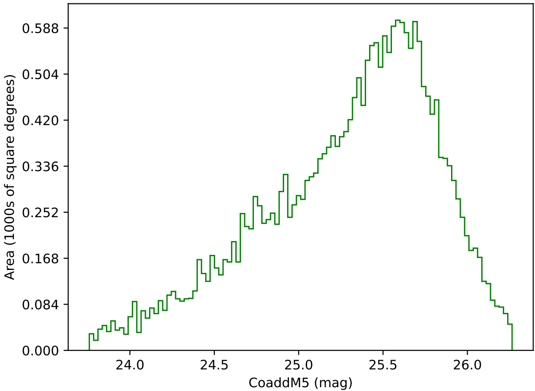
too_elab_heavy_r128_d2_griz_v3.4_10yrs Yr 3-4 g band: CoaddM5
