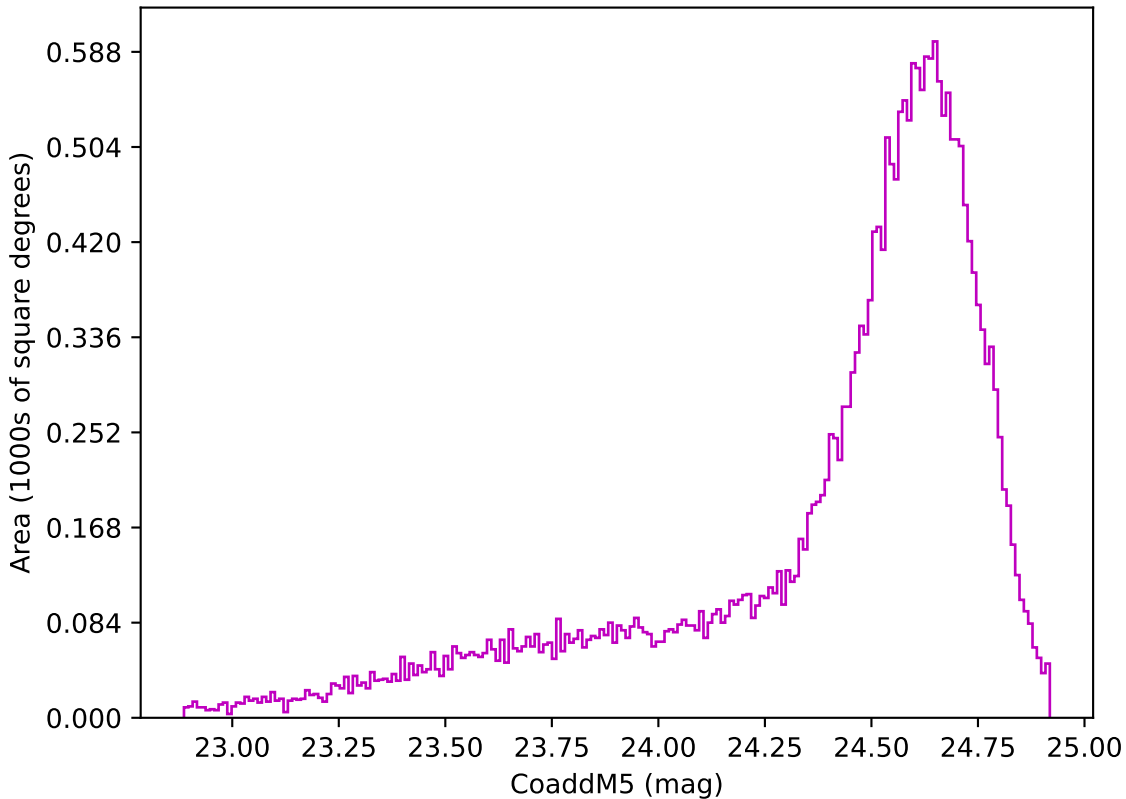
too_elab_heavy_r128_d2_griz_v3.4_10yrs Yr 1 z band: CoaddM5
