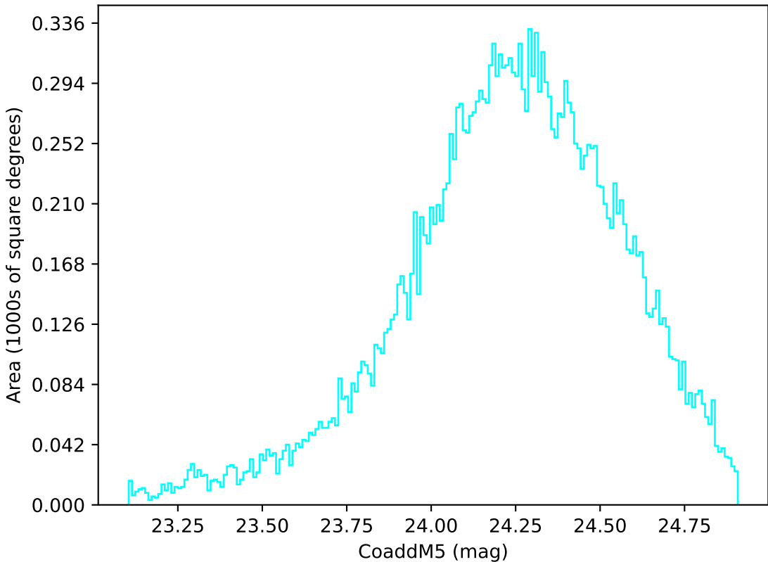
too_elab_heavy_r128_d2_griz_v3.4_10yrs Yr 1 u band: CoaddM5
