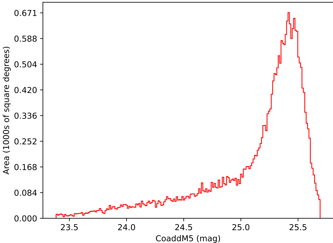
too_elab_heavy_r128_d2_griz_v3.4_10yrs Yr 1 i band: CoaddM5
