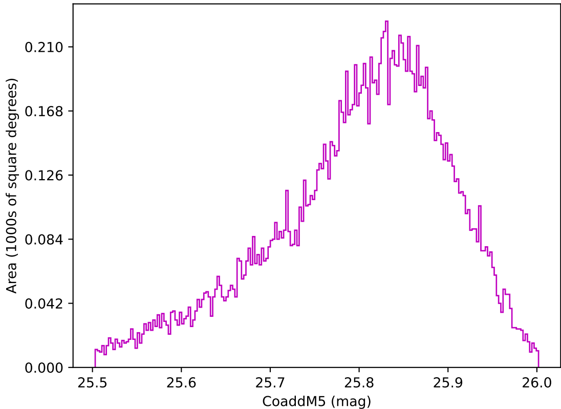
too_elab_heavy_r128_d2_griz_v3.4_10yrs WFD z band: CoaddM5
