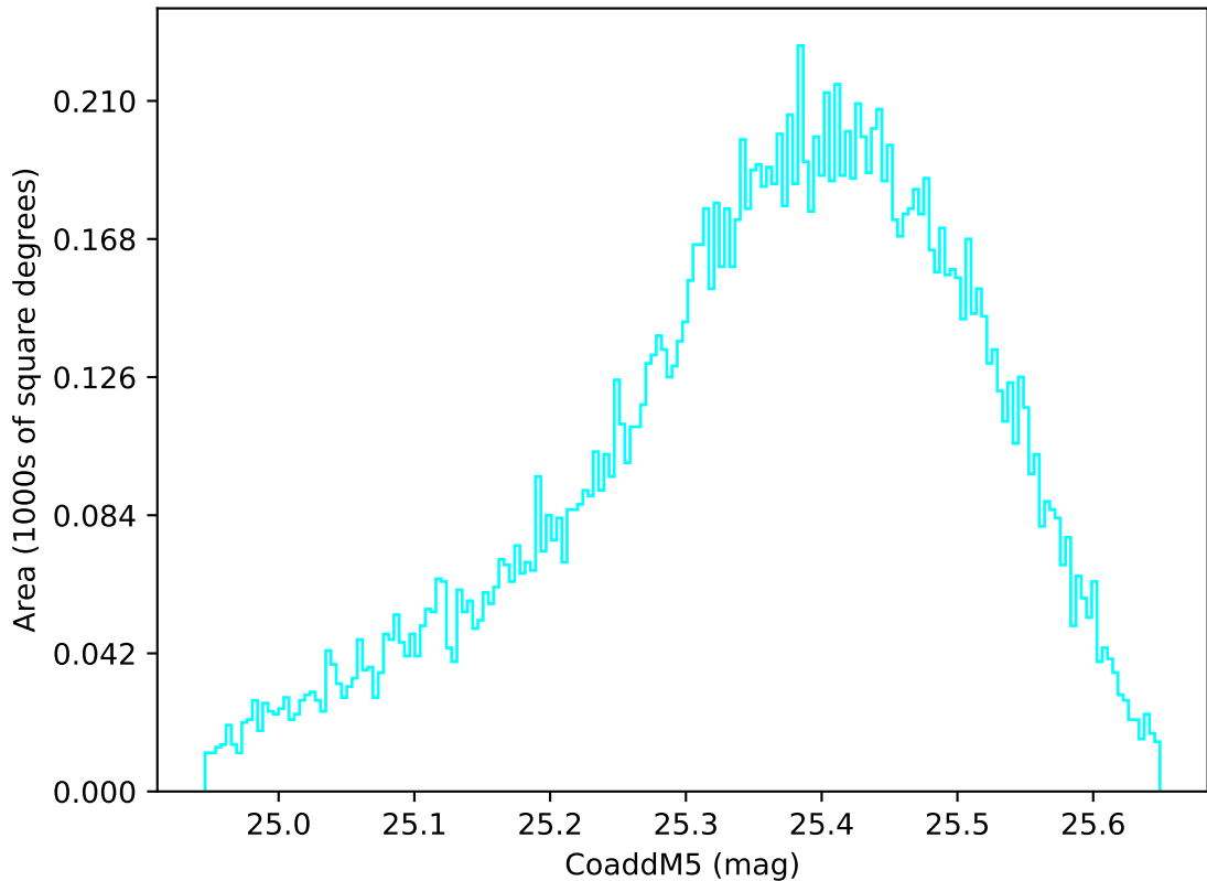
too_elab_heavy_r128_d2_griz_v3.4_10yrs WFD u band: CoaddM5
