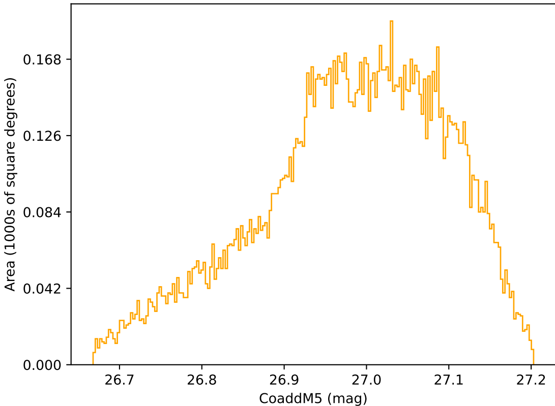
too_elab_heavy_r128_d2_griz_v3.4_10yrs WFD r band: CoaddM5
