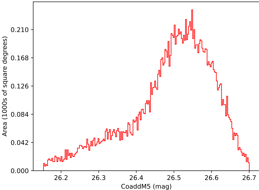
too_elab_heavy_r128_d2_griz_v3.4_10yrs WFD i band: CoaddM5
