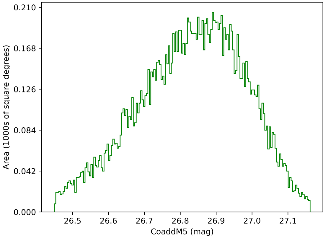
too_elab_heavy_r128_d2_griz_v3.4_10yrs WFD g band: CoaddM5
