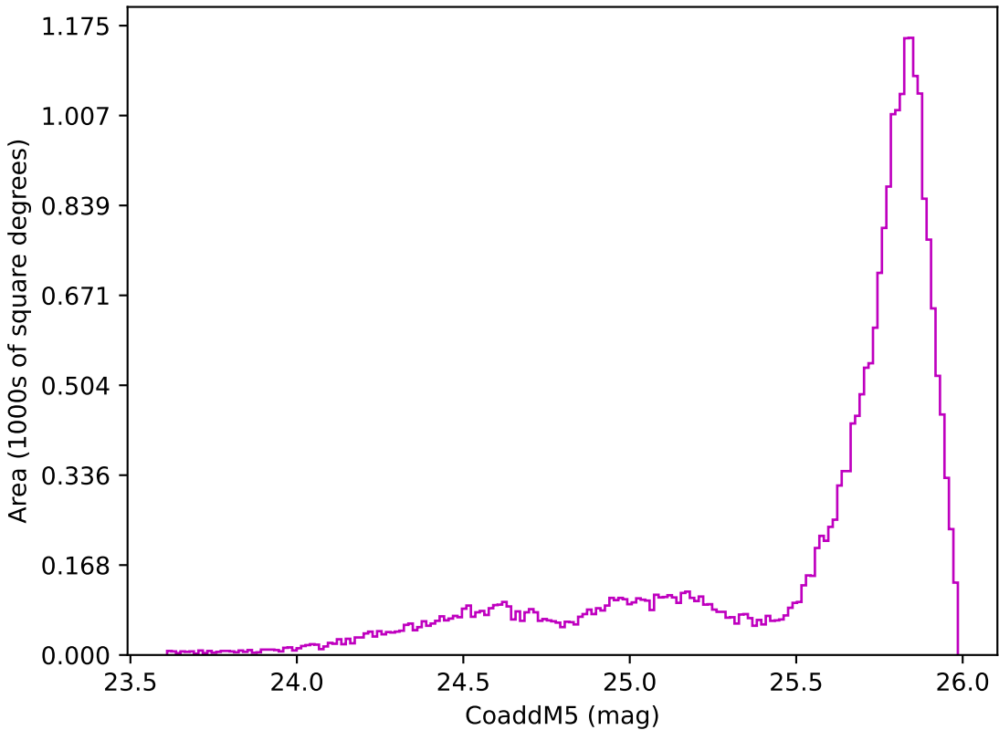
too_elab_heavy_r128_d2_griz_v3.4_10yrs All sky z band: CoaddM5
