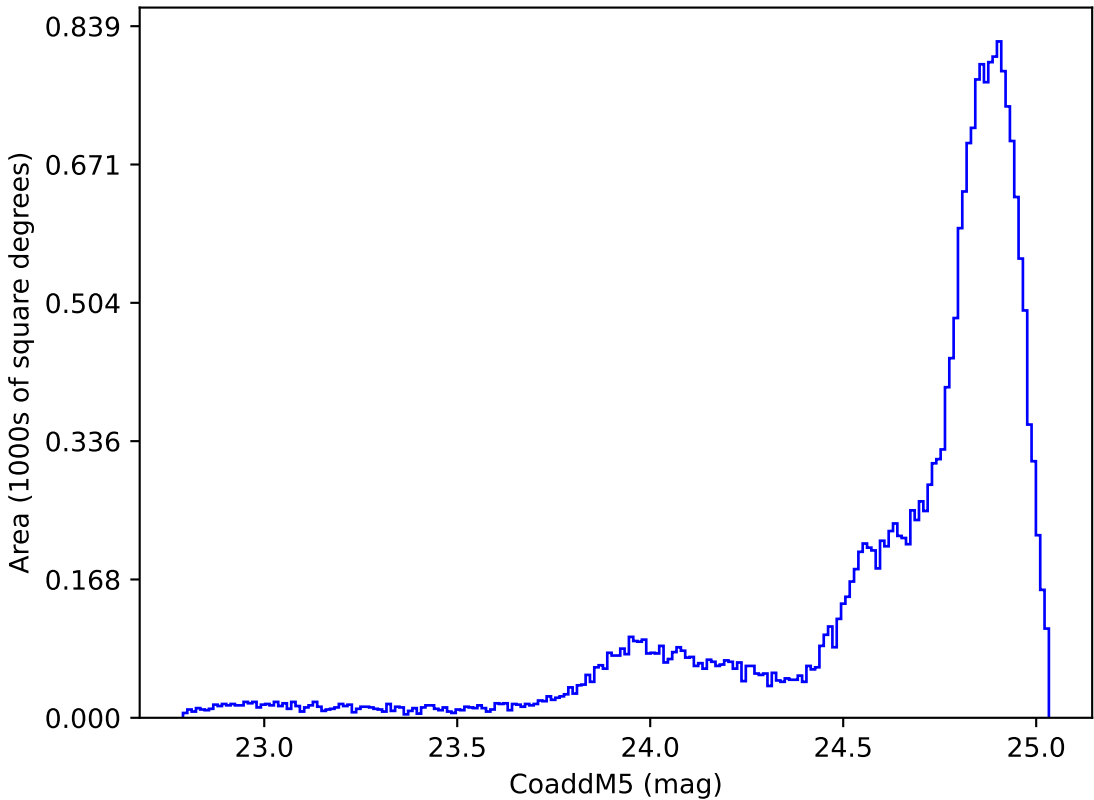
too_elab_heavy_r128_d2_griz_v3.4_10yrs All sky y band: CoaddM5
