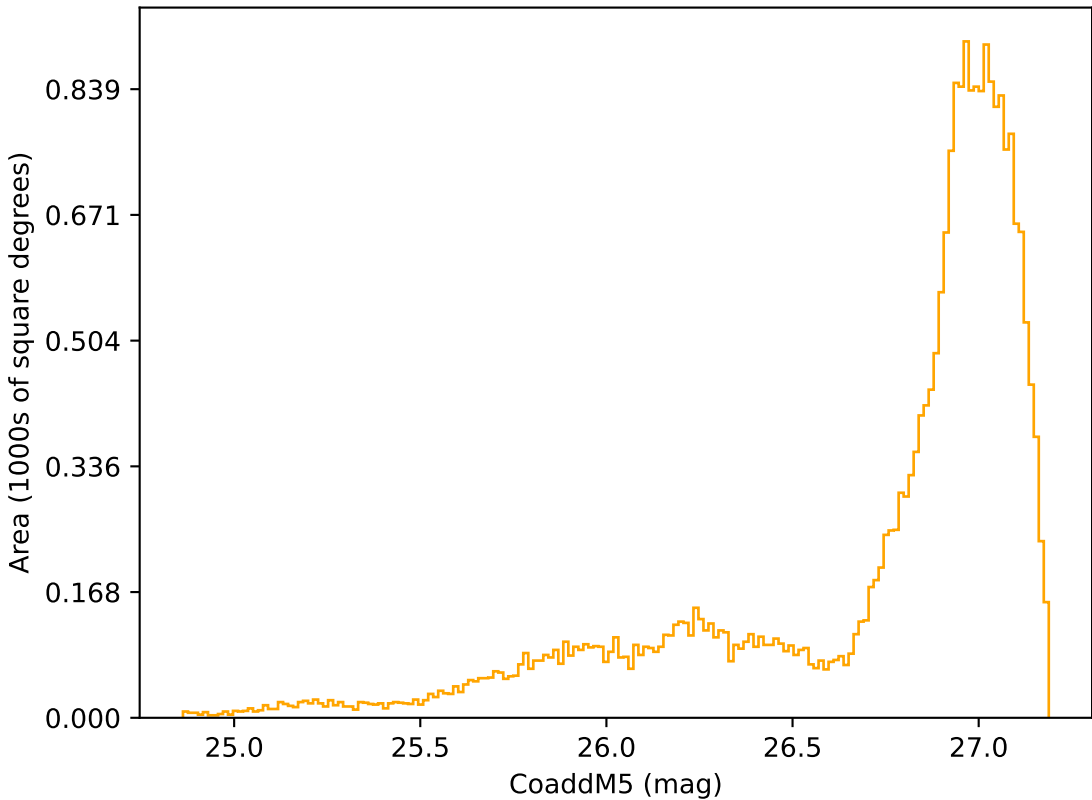
too_elab_heavy_r128_d2_griz_v3.4_10yrs All sky r band: CoaddM5
