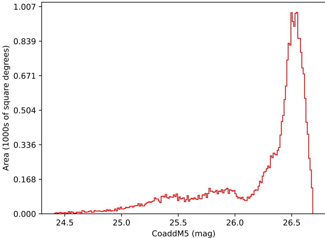
too_elab_heavy_r128_d2_griz_v3.4_10yrs All sky i band: CoaddM5
