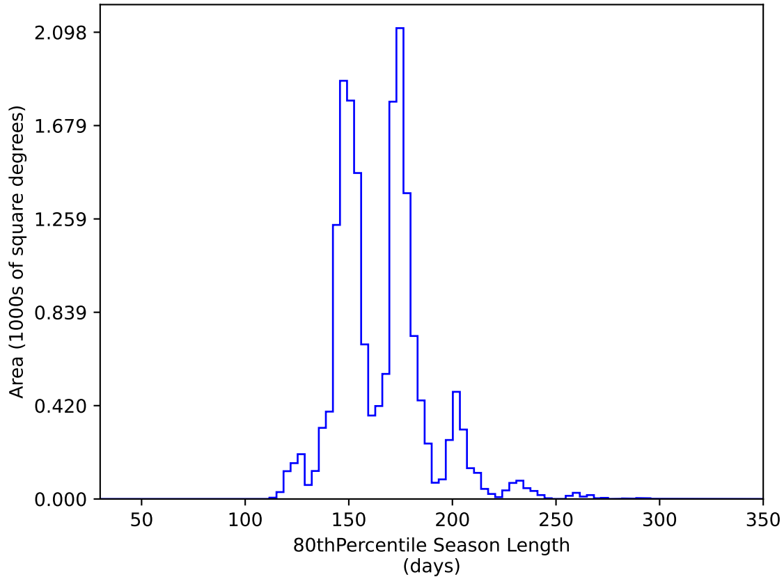
too_elab_heavy_r128_d2_griz_v3.4_10yrs WFD y band: 80thPercentile Season Length
