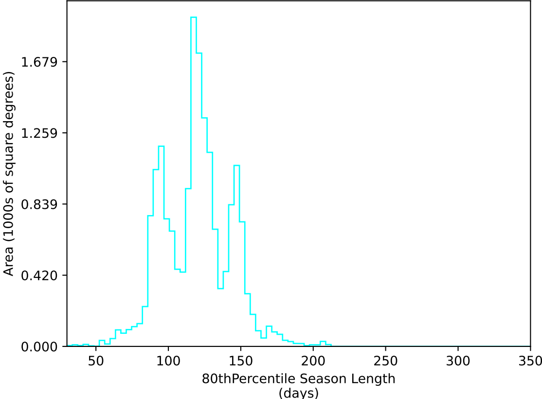
too_elab_heavy_r128_d2_griz_v3.4_10yrs WFD u band: 80thPercentile Season Length
