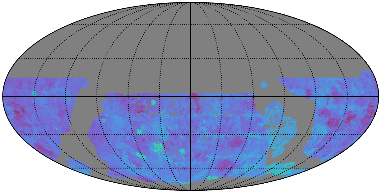
too_elab_heavy_r128_d2_griz_v3.4_10yrs WFD g band: 80thPercentile Season Length
