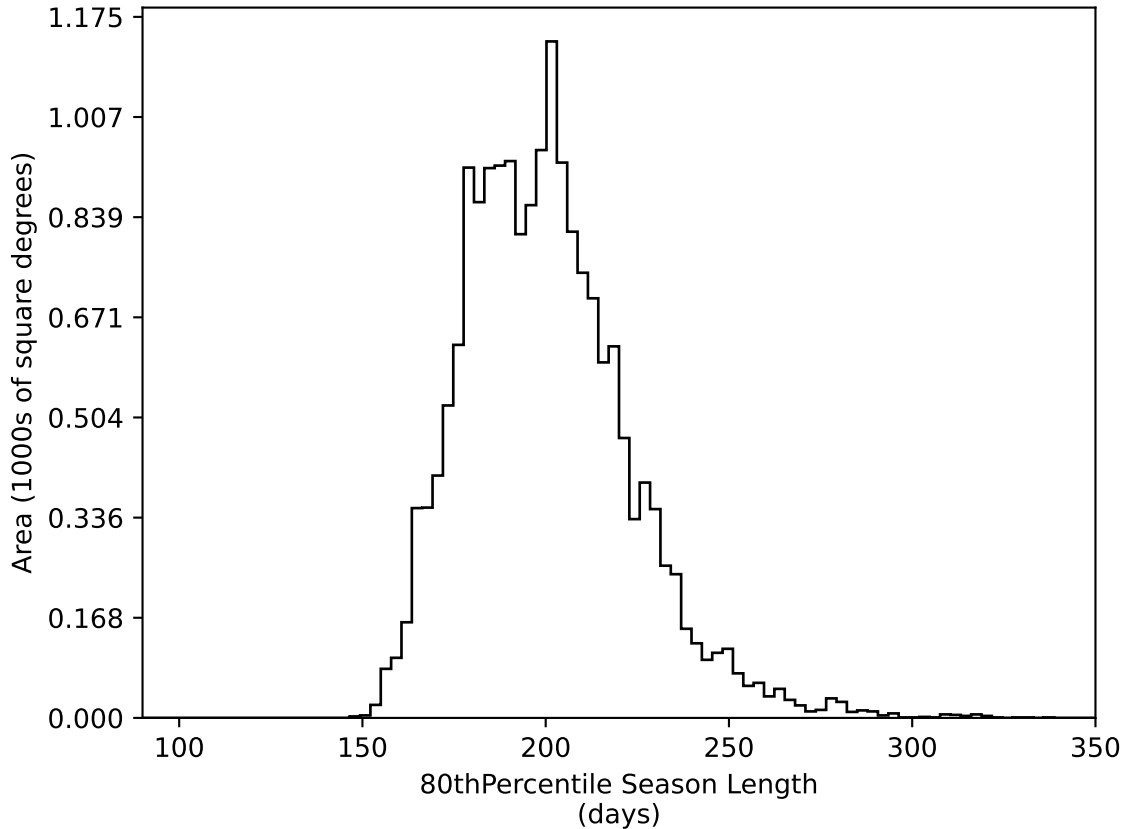
too_elab_heavy_r128_d2_griz_v3.4_10yrs WFD all bands: 80thPercentile Season Length
