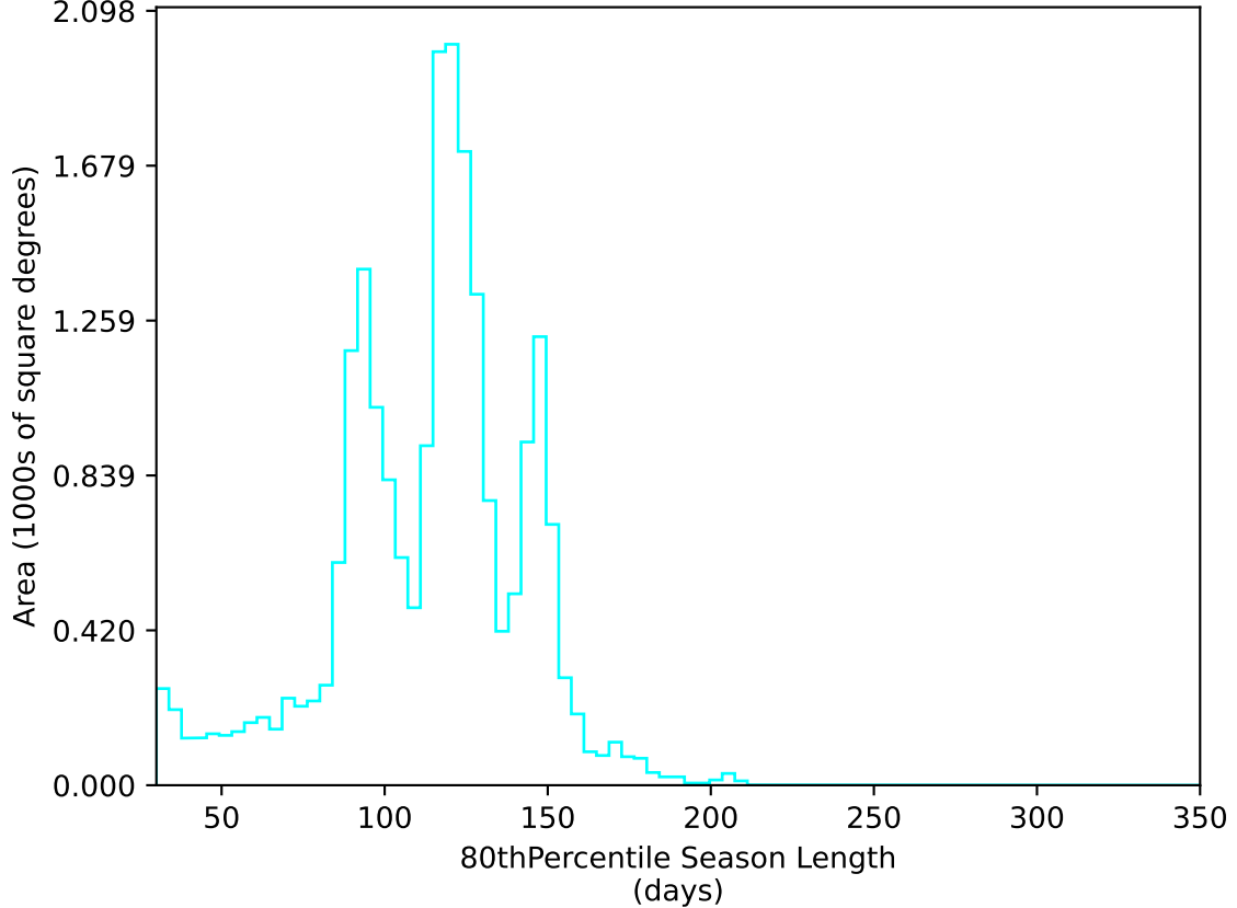
too_elab_heavy_r128_d2_griz_v3.4_10yrs All sky u band: 80thPercentile Season Length
