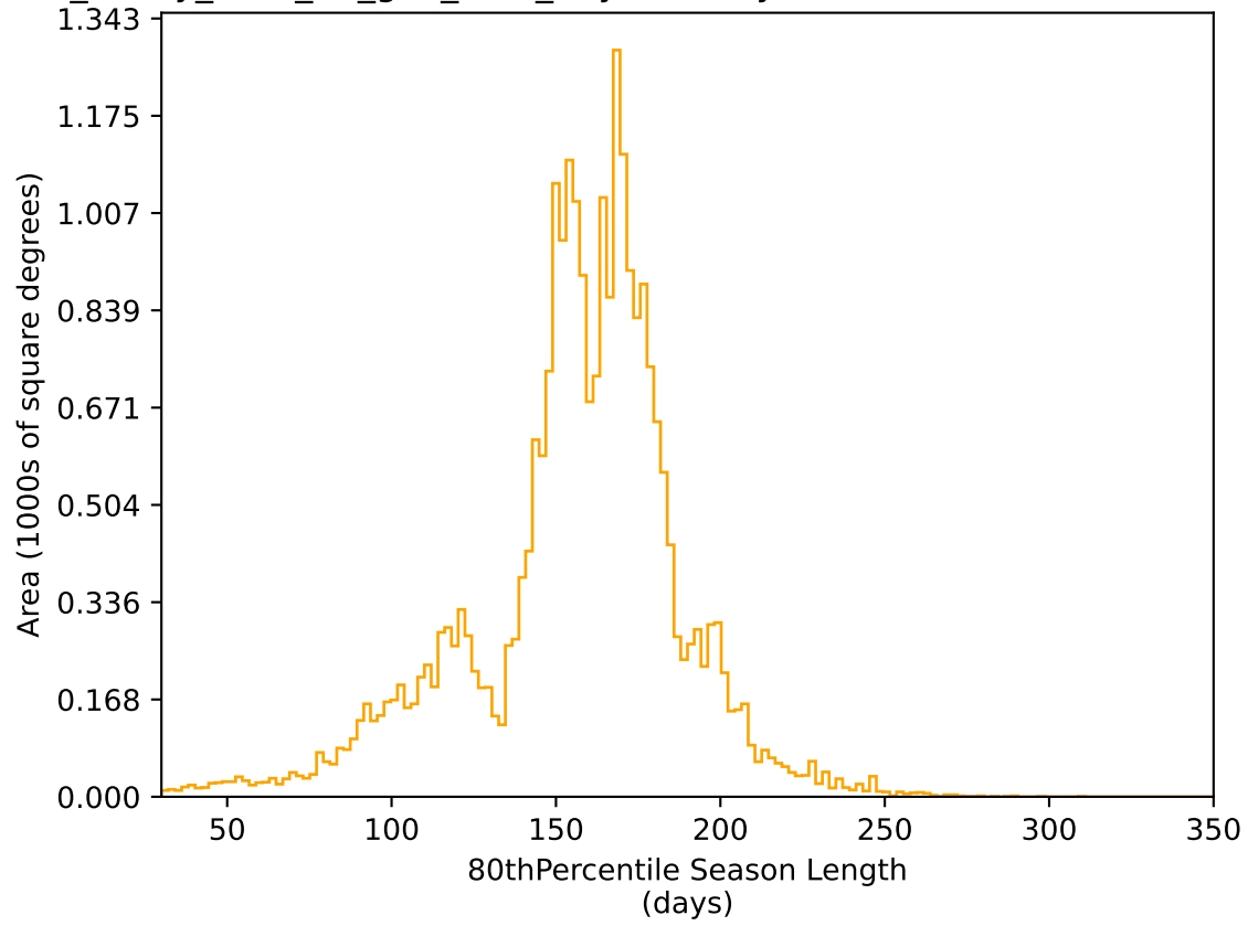
too_elab_heavy_r128_d2_griz_v3.4_10yrs All sky r band: 80thPercentile Season Length
