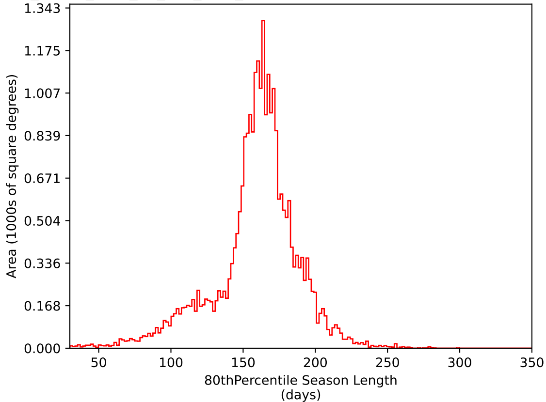
too_elab_heavy_r128_d2_griz_v3.4_10yrs All sky i band: 80thPercentile Season Length
