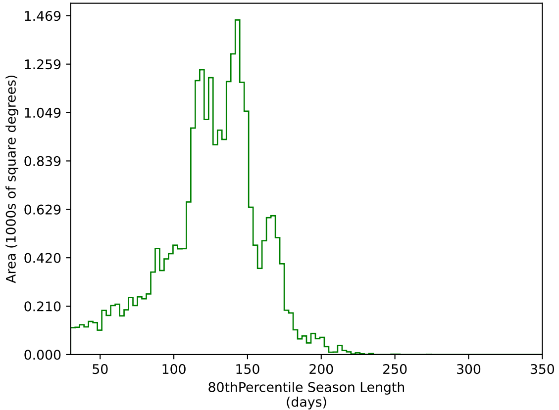
too_elab_heavy_r128_d2_griz_v3.4_10yrs All sky g band: 80thPercentile Season Length
